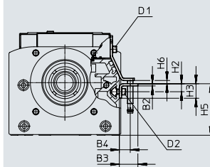
Sensor bracket HWS-EGC
