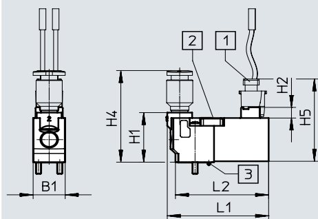
Plug connection on top
