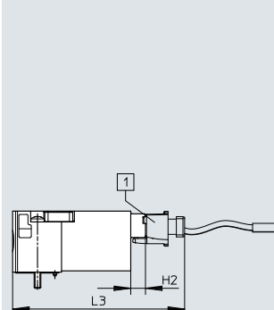
Plug connection at the rear
