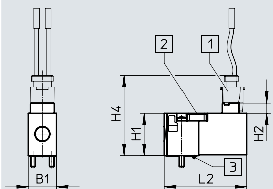
Plug connection on top
