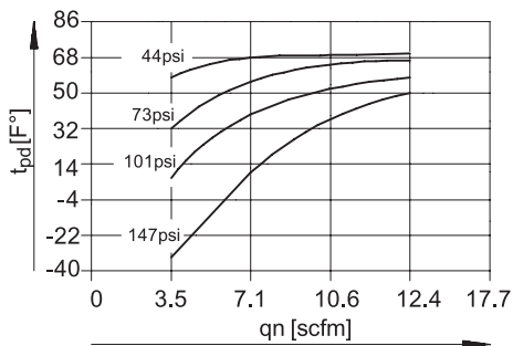
Pressure dew point t pd (outlet) as a function of the standard flow rate at outlet q n (MS6N-LDM1-...-P20)
