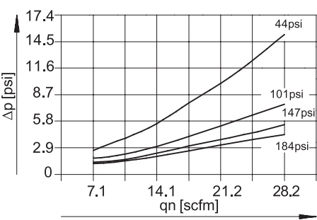
Differential pressure \Delta p as a function of the standard flow rate at outlet q_n (MS6N-LDM1-...-P40)
