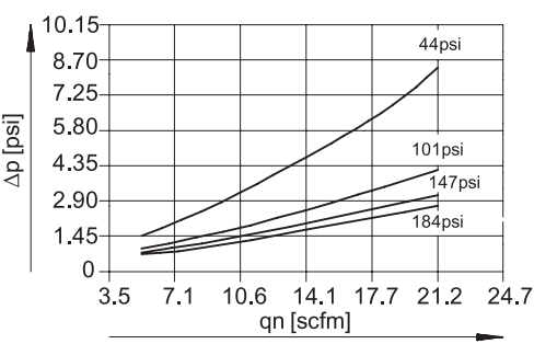
Differential pressure \Delta p as a function of the standard flow rate at outlet q_n (MS6N-LDM1-...-P30)
