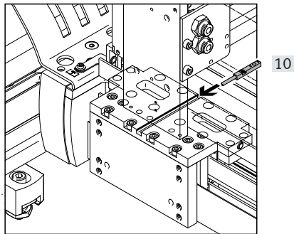
Proximity switch for sensing the position of the slide on the Y-axis
