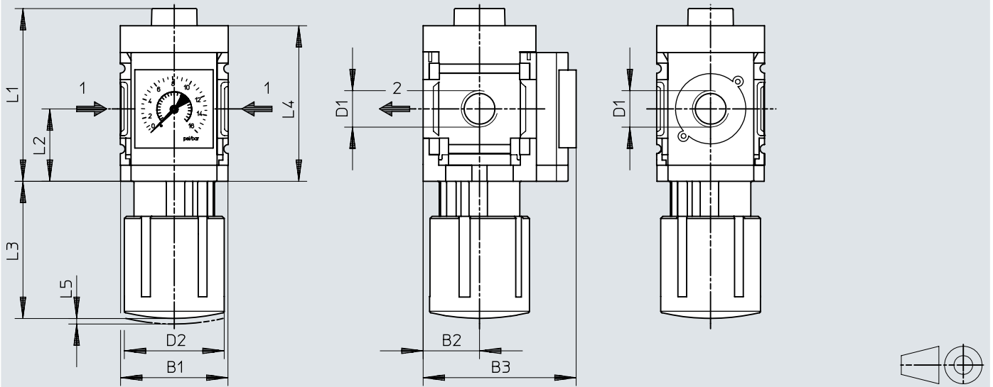
Dimensions – Alternative mounting position, rotary knob at the bottom
